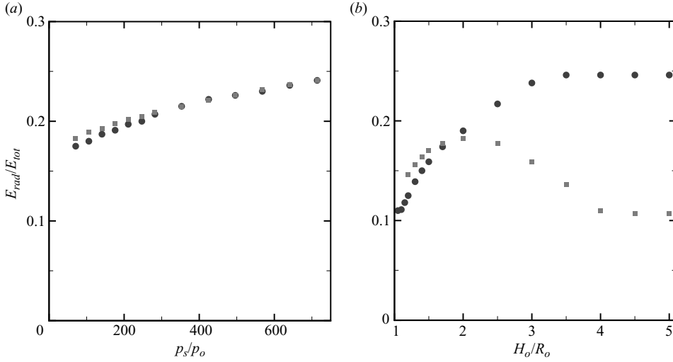
FIGURE 19. Fraction of the radiated energy for shock-induced (squares) and Rayleigh (circles) collapse: (a) free-field collapse; (b) collapse near a wall. Shock-induced collapse: p_s/p_o = 353 ; Rayleigh collapse: p_s/p_o = 714 .
