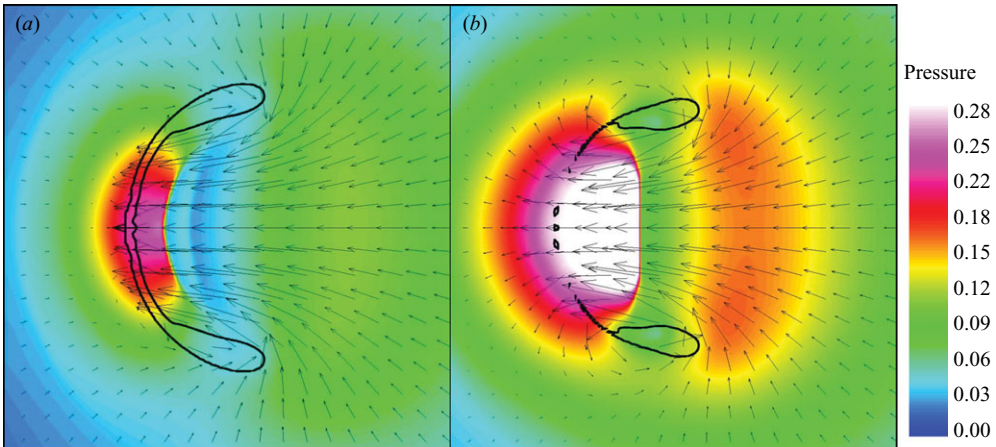
FIGURE 18. Pressure contours non-dimensionalized by \rho_L c_L^2 (approximate interface location: \gamma = 1.42 contour) and velocity vectors showing the water-hammer shock in free-field shock-induced collapse ( p_s/p_o = 353 ) at times (a) t/(R_o/c_L) = 8.49 , (b) t/(R_o/c_L) = 8.68 .
