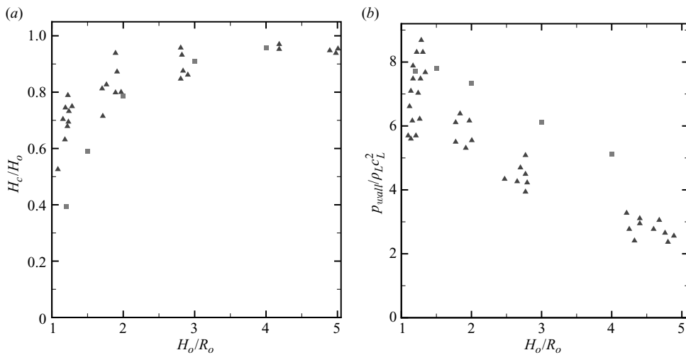
FIGURE 24. Comparison of shock-induced collapse near a wall with p_s/p_o = 25 between the present simulations (squares) and the experiments by Shima et al. (1984) (triangles): (a) Distance between the wall and the bubble at collapse; (b) wall pressure averaged over the area of the hydrophone used in the experiment.
