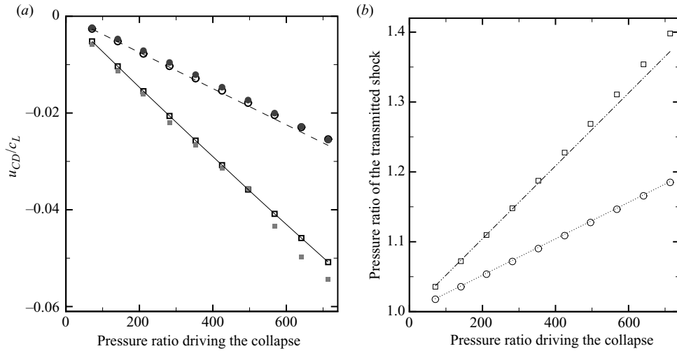
FIGURE 7. Initial interface velocity, and pressure ratio across the transmitted shock as a function of the pressure ratio driving the collapse for shock-induced (squares) and Rayleigh (circles) collapse. The open symbols denote the analytical solution to the corresponding planar Riemann problem and the filled symbols refer to the simulations. (a) Initial interface velocity. Dashed line: (3.2); solid line: (3.3). (b) Pressure ratio across the transmitted shock. Dotted line: 1 + \alpha z ; dashed-dotted line: 1 + 2\alpha z .
