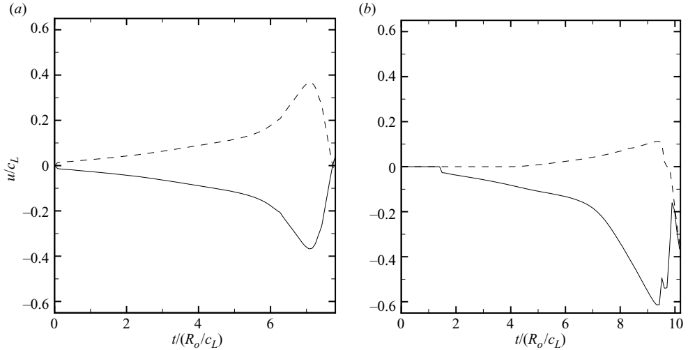
FIGURE 8. History of the velocity of the jet (solid line) and of the distal side (dashed line) for free-field collapse ( p_s/p_o = 353 ). (a) Rayleigh collapse and (b) shock-induced collapse.
