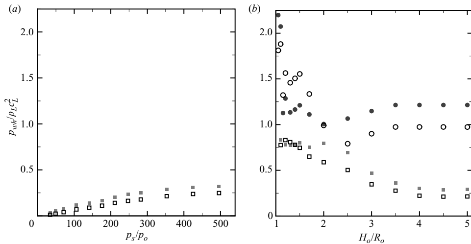
FIGURE 16. Water-hammer pressure for shock-induced (square) and Rayleigh (circles) collapse. The empty symbols denote the values computed from (5.1) and the filled symbols are the values measured in the simulations: (a) free-field collapse; (b) collapse near a wall. Shock-induced collapse: p_s/p_o = 353 ; Rayleigh collapse: p_s/p_o = 714 .
