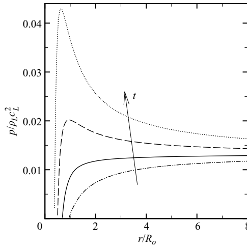
FIGURE 9. Pressure in the liquid as a function of distance at different times using (3.4) for Rayleigh collapse ( p_s/p_o = 353 ). Dashed-dotted line: t/(R_o/c_L) = 2.88 ; solid line: t/(R_o/c_L) = 6.17 ; dashed line: t/(R_o/c_L) = 7.19 ; dotted line: t/(R_o/c_L) = 7.60 .
