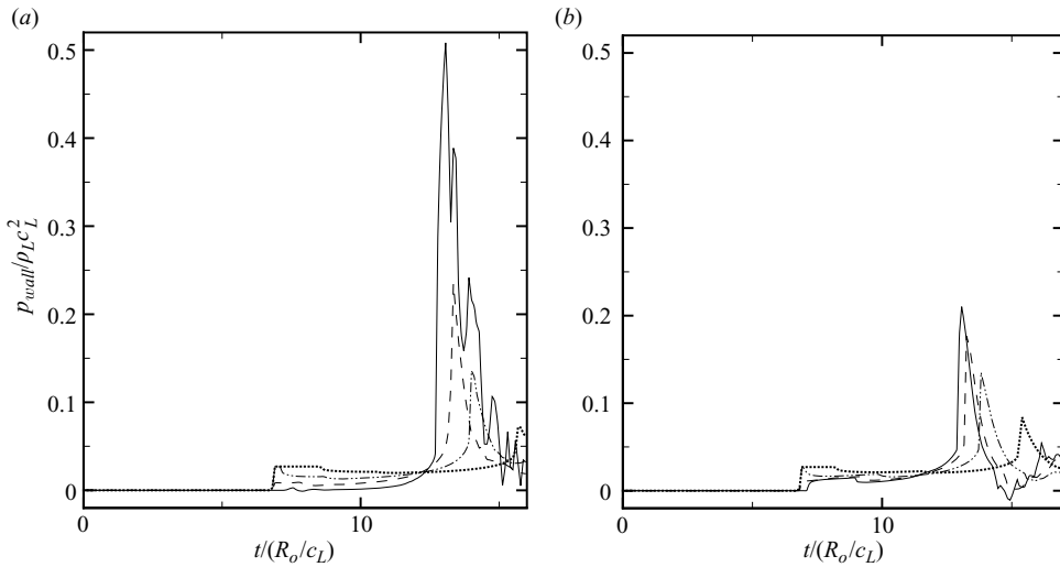
FIGURE 21. History of the wall pressure at different locations along the wall for shock-induced collapse near a wall ( p_s/p_o = 353 ): (a) H_o/R_o = 1.2 ; (b) H_o/R_o = 2.0 . Solid line: s/R_o = 0.0 ; dashed line: s/R_o = 1.0 ; dashed-dotted line: s/R_o = 2.0 ; dotted line: s/R_o = 4.0 .
