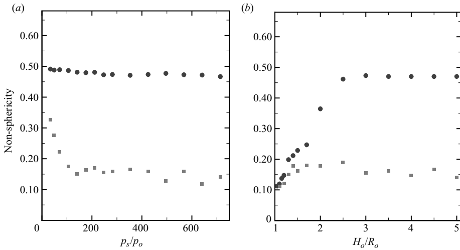
FIGURE 12. Maximum bubble non-sphericity for shock-induced (squares) and Rayleigh (circles) collapse. The non-sphericity is given by the ratio of the projected bubble area to the length of the perimeter normalized by the average radius; a value of 0.5 corresponds to a spherical collapse. The maximum value is achieved at collapse: (a) free-field collapse; (b) collapse near a wall. Shock-induced collapse: p_s/p_o = 353 ; Rayleigh collapse: p_s/p_o = 714 .
