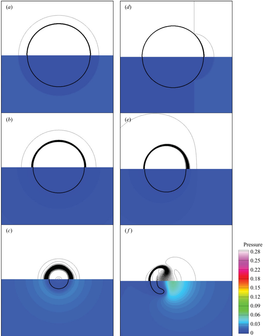
FIGURE 4. Evolution of free-field collapse ( p_s/p_o = 353 ): (a) Rayleigh collapse at times (a) t/(R_o/c_L) = 0.265 , (b) t/(R_o/c_L) = 3.98 , (c) t/(R_o/c_L) = 6.98 and (b) shock-induced collapse at times (d) t/(R_o/c_L) = 0.280 , (e) t/(R_o/c_L) = 5.79 , (f) t/(R_o/c_L) = 8.02 . Top: density lines; bottom: pressure contours non-dimensionalized by \rho_L c_L^2 (approximate interface location: \gamma = 1.42 contour).
