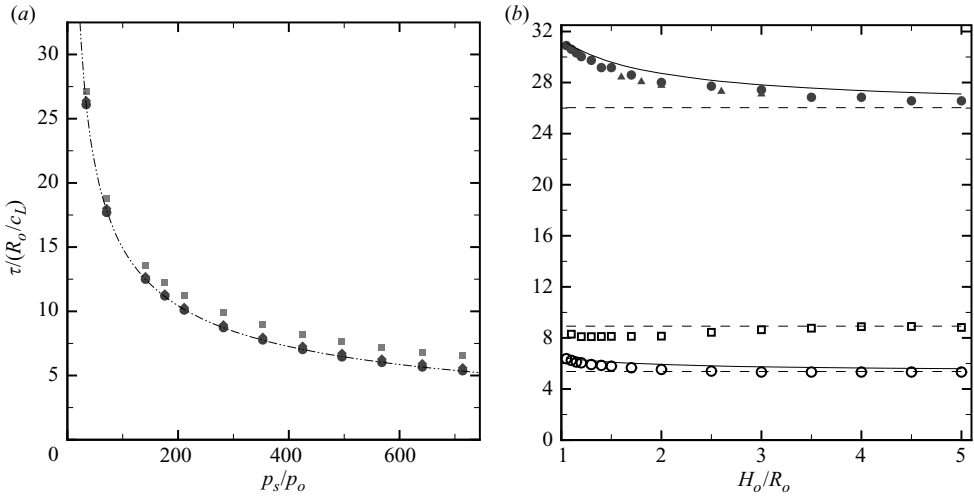
FIGURE 10. Collapse time for shock-induced (squares) and Rayleigh (circles) collapse. (a) Free-field collapse. Diamonds: solution from the Rayleigh–Plesset equation for spherical collapse; dashed-dotted line: \sim 1/\sqrt{p_s/p_o - 1} . (b) Collapse near a wall. Triangles: experiments by Lindau & Lauterborn (2003); solid line: \tau_r ; dashed line: \tau_c . The filled symbols denote cavitation conditions ( p_s/p_o = 34 ) and the open symbols indicate shock wave lithotripsy conditions (shock-induced collapse: p_s/p_o = 353 ; Rayleigh collapse: p_s/p_o = 714 ).
