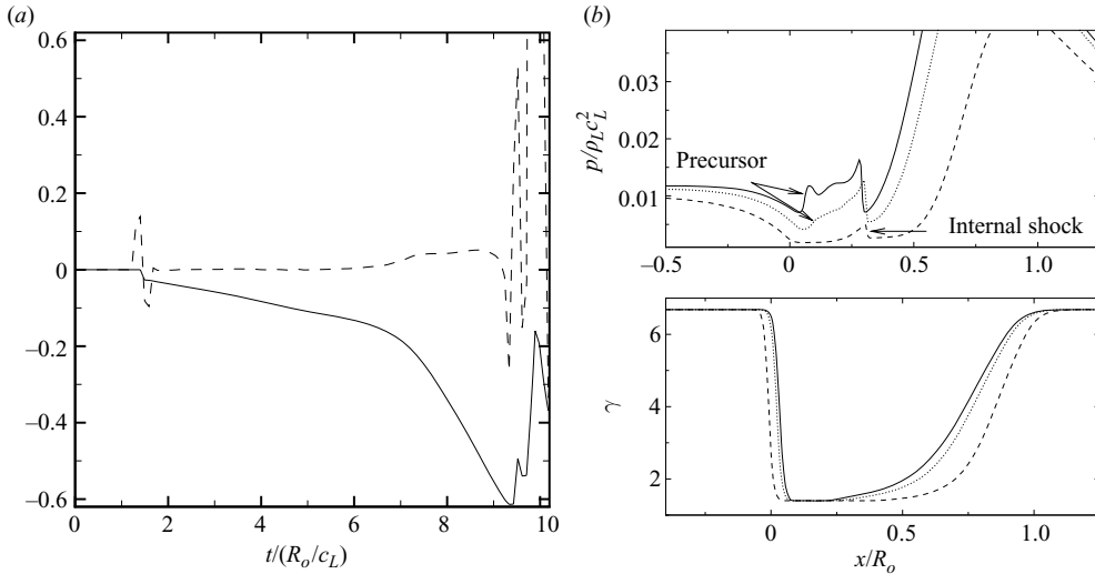
FIGURE 14. Formation of the precursor shock in free-field shock-induced collapse. (a) History of the jet velocity (solid line) and of the left-hand side of equation 4.3 (dashed line). (b) Pressure (top) and \gamma (bottom) profiles along the centreline. Dashed line: t/(R_o/c_L)=9.24 ; dotted line: t/(R_o/c_L)=9.52 ; solid line: t/(R_o/c_L)=9.61 .
