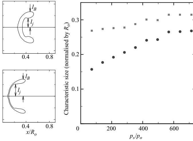
FIGURE 13. Characteristic lengths in free-field shock-induced collapse. The characteristic size of the jet is taken as the length between the x -axis and the point where the jet outline first becomes horizontal, and the bubble height is the distance between the centreline and the topmost part of the bubble at that instant: (a) Jet outline. Top: p_s/p_o = 71 at t/(R_o/c_L) = 20.1 ; bottom: p_s/p_o = 282 at t/(R_o/c_L) = 11.0 . (b) Characteristic lengths as a function of pressure ratio across the shock. Circles: jet size, l_j ; squares: bubble height, l_B .
