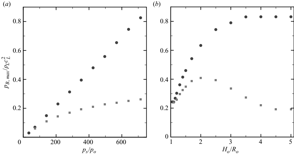
FIGURE 20. Maximum average bubble pressure for shock-induced (squares) and Rayleigh (circles) collapse: (a) free-field collapse; (b) collapse near a wall. Shock-induced collapse: p_s / p_o = 353 ; Rayleigh collapse: p_s / p_o = 714 .
