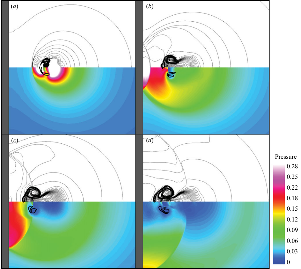
FIGURE 22. Collapse and shock propagation in shock-induced collapse near a wall with p_s/p_o = 353 , H_o/R_o = 1.5 at times (a) t/(R_o/c_L) = 7.93 , (b) t/(R_o/c_L) = 8.58 , (c) t/(R_o/c_L) = 8.96 , (d) t/(R_o/c_L) = 9.42 . Top: density lines; bottom: pressure contours non-dimensionalized by \rho_L c_L^2 (approximate interface location: \gamma = 1.42 contour).
